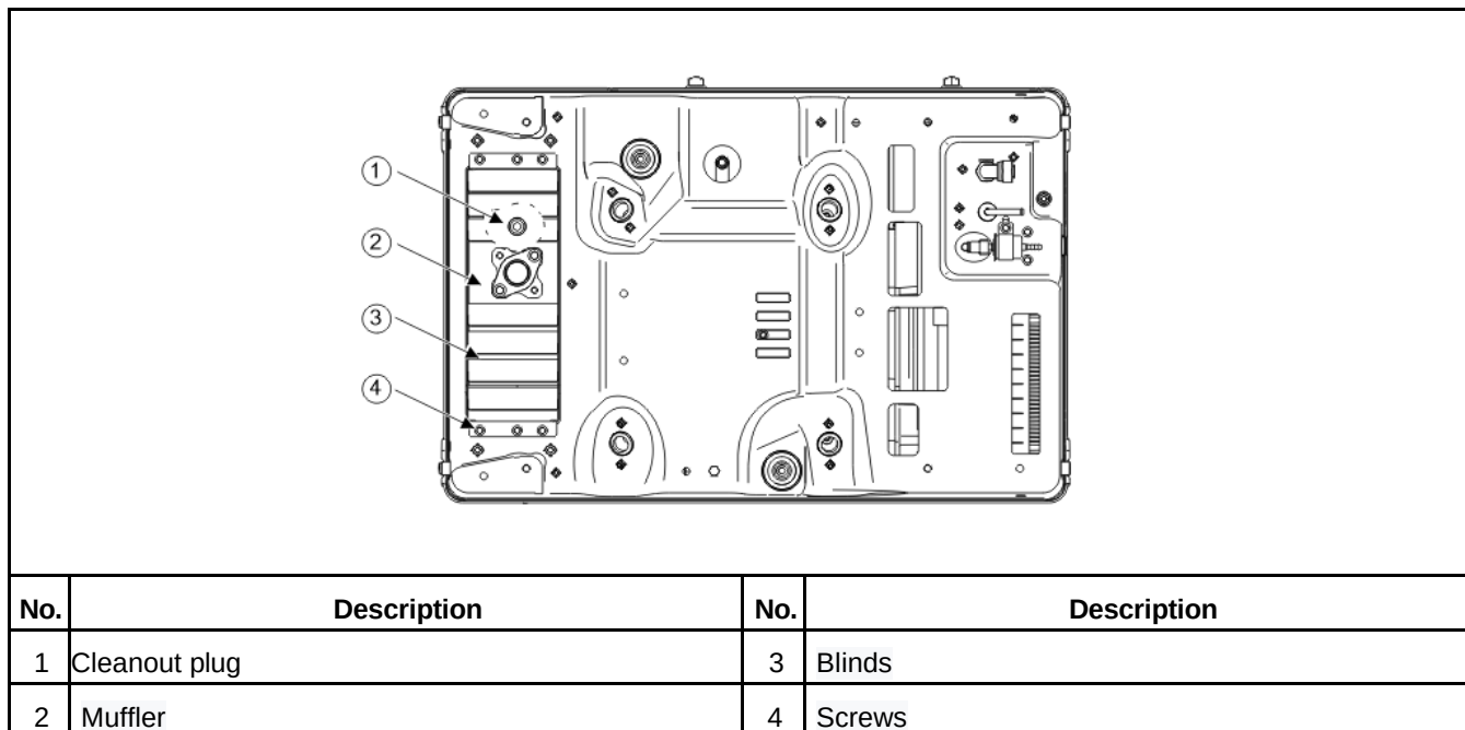
FIGURE 13. SPARK ARRESTER CLEANOUT PLUG
